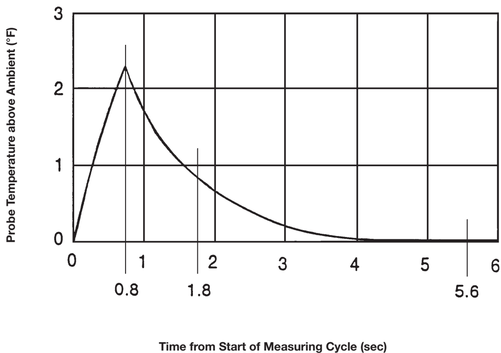
Typical Flow Measuring Cycle
